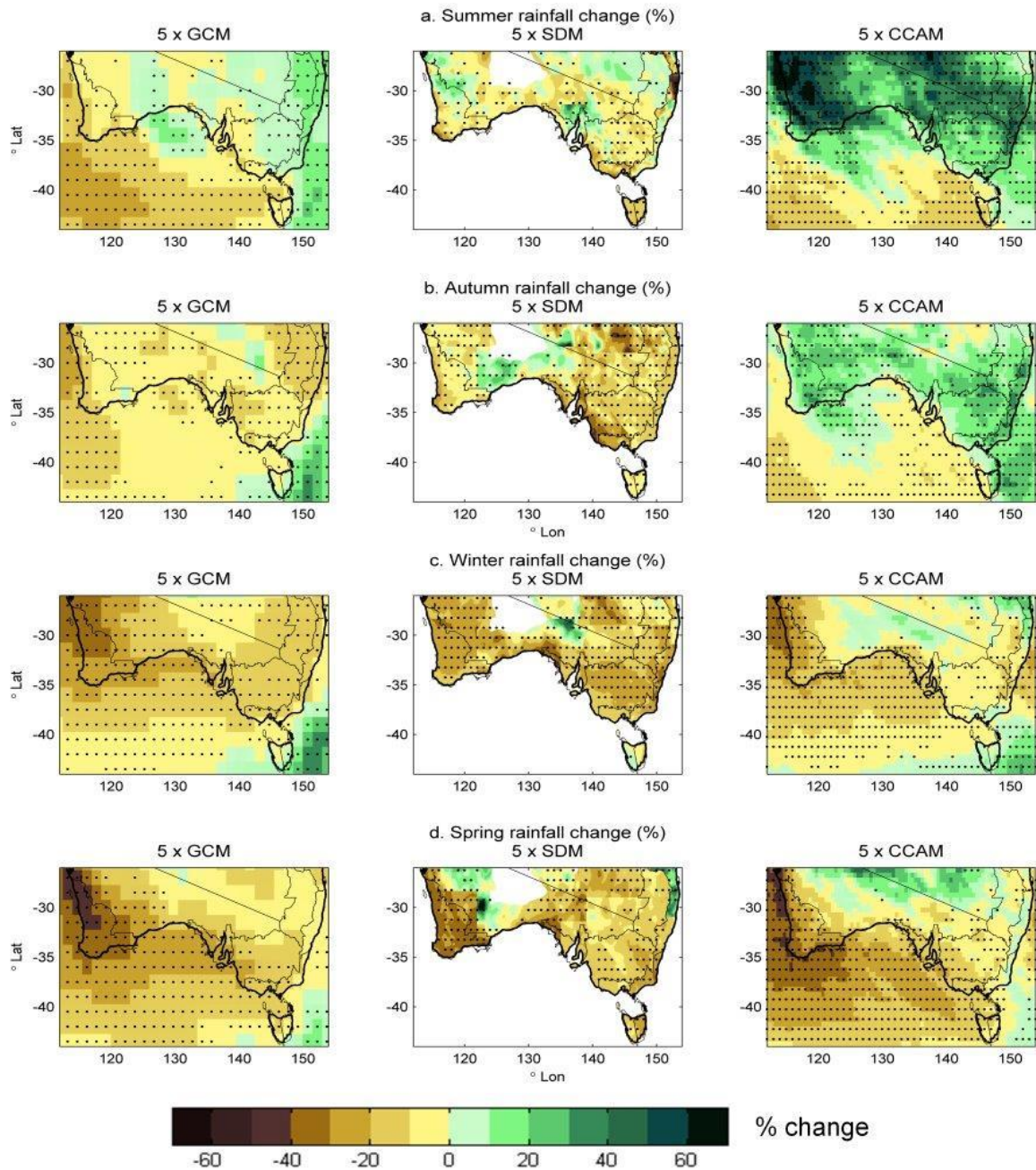
Figure 10 Projected rainfall changes (%) in southern Australia from 5 CMIP5 GCMs, and BOM-SDM and CCAM downscaling using those same five GCMs as input (see Table 1) for 1986-2005 to 2080-2099 under RCP8.5. Stippling indicates where four or five models agree on the sign of change. Note that summer is in the top row, then autumn etc. unlike Figure 9. The white regions in BOM-SDM results indicate an area with insufficient observed data coverage to use in the model.
