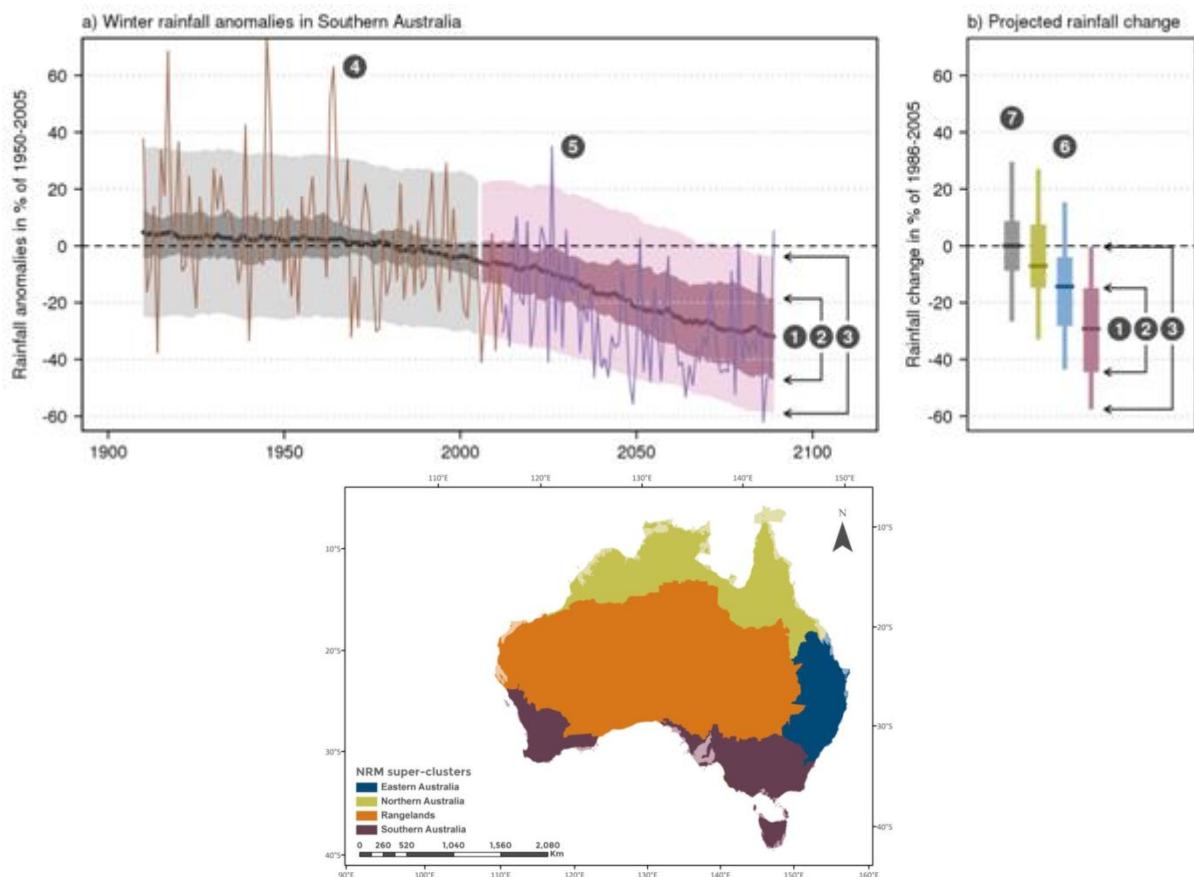
Figure 1 Time series of observed and simulated rainfall change (a) and projected change according to different scenarios (b) for winter (JJA) rainfall in Southern Australia (see region shaded purple in inset map). The range of model results is summarised using the median (1) and 10th to 90th percentile range of the projected change (2) in all available CMIP5 simulations. The change in mean climate is shown as 20-year moving averages. Dark shading (2) indicates the 10th to 90th percentile range for 20-year averages, whilst light shading (3) indicates change in the 10th to 90th percentile for individual years. The AWAP time series of each year (4) is overlaid to enable comparison between observed variability and simulated model spread, while the variability from one climate model (ACCESS1.0) is shown for the future period (5). The reference period in (a) is 1950–2005, to avoid ‘pinching’ of the model range around a narrow recent time window, while the bar graphs (b) are the difference between two periods: 2080–2099 minus 1986–2005 for green: RCP2.6, blue: RCP4.5, purple: RCP8.5 (6) and grey: natural variability only (7). (Source: NRM Technical Report: CSIRO and Bureau of Meteorology, 2015)
